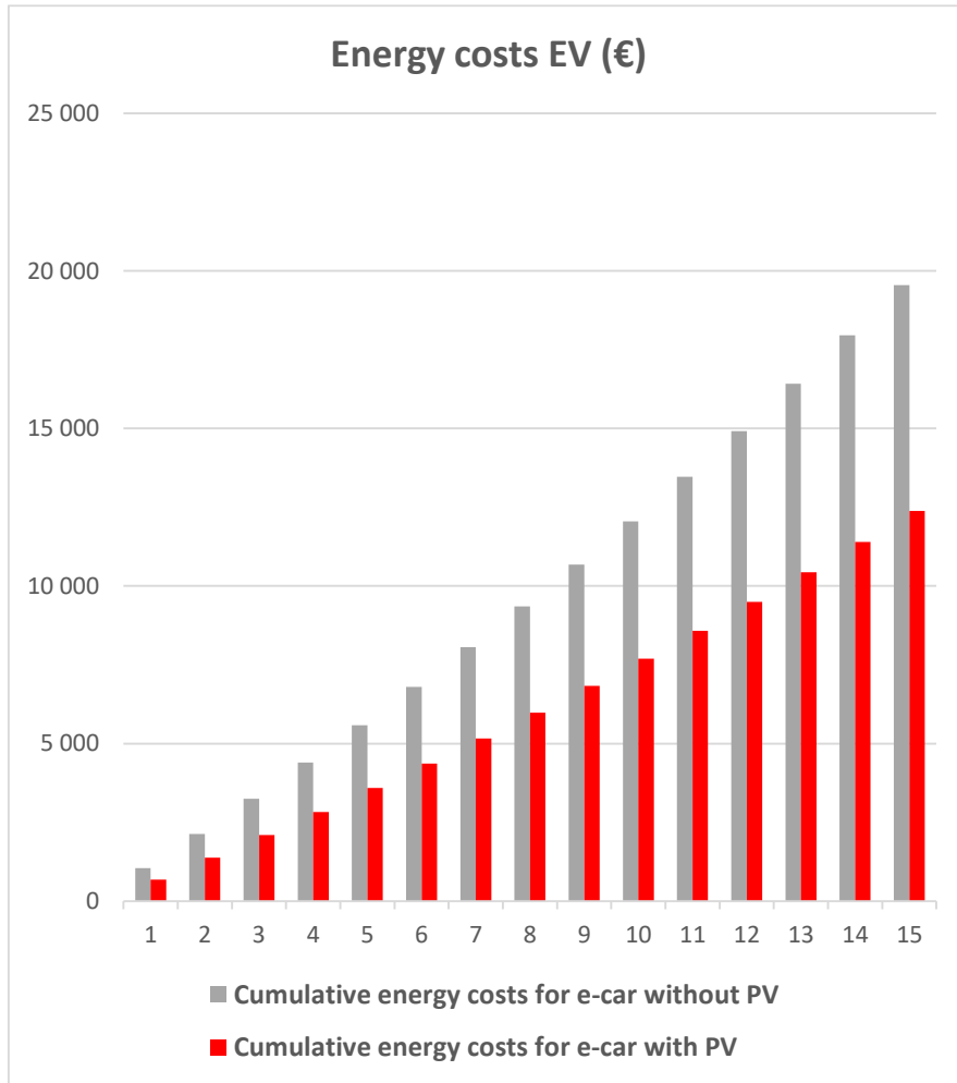
Figure 10: Cumulative energy costs for an electric car with and without PV system
