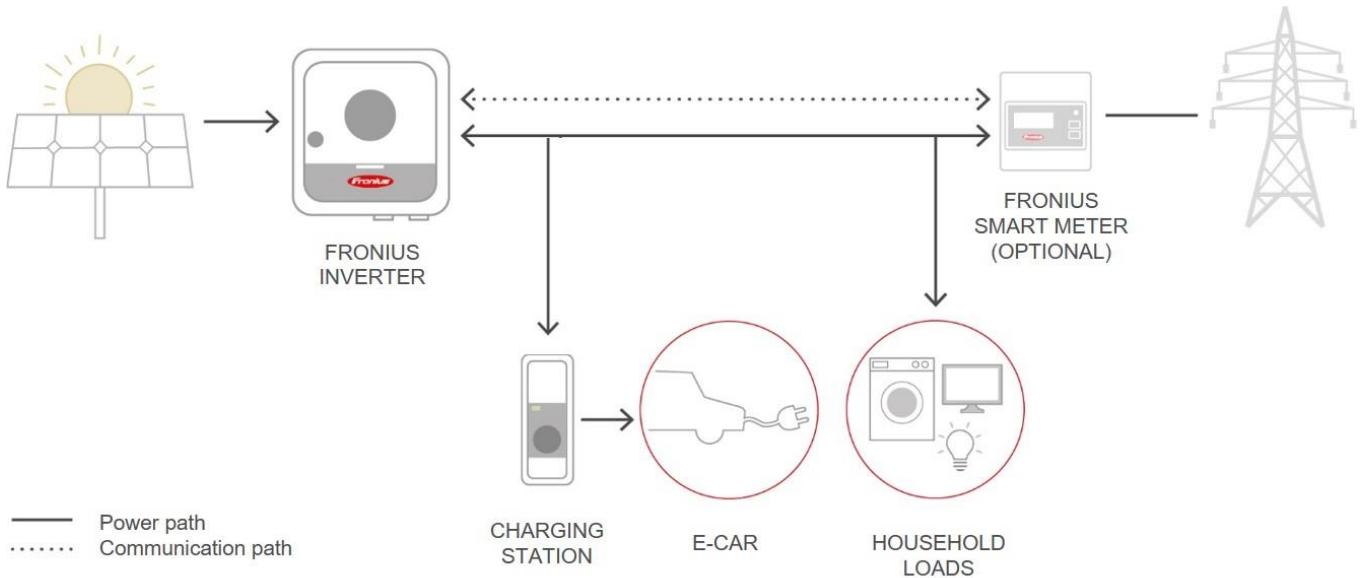
Figure 14: Configuration diagram 'manual charging with PV energy'
